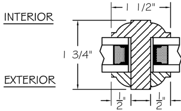
TRUE DIVIDED LITE BAR (OVOLO STICKING)
