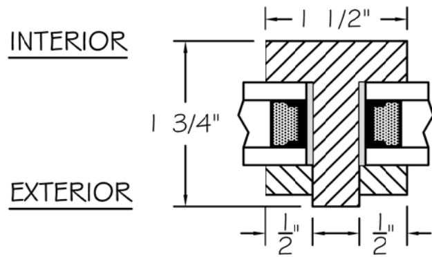
TRUE DIVIDED LITE BAR (SQUARE STICKING)
